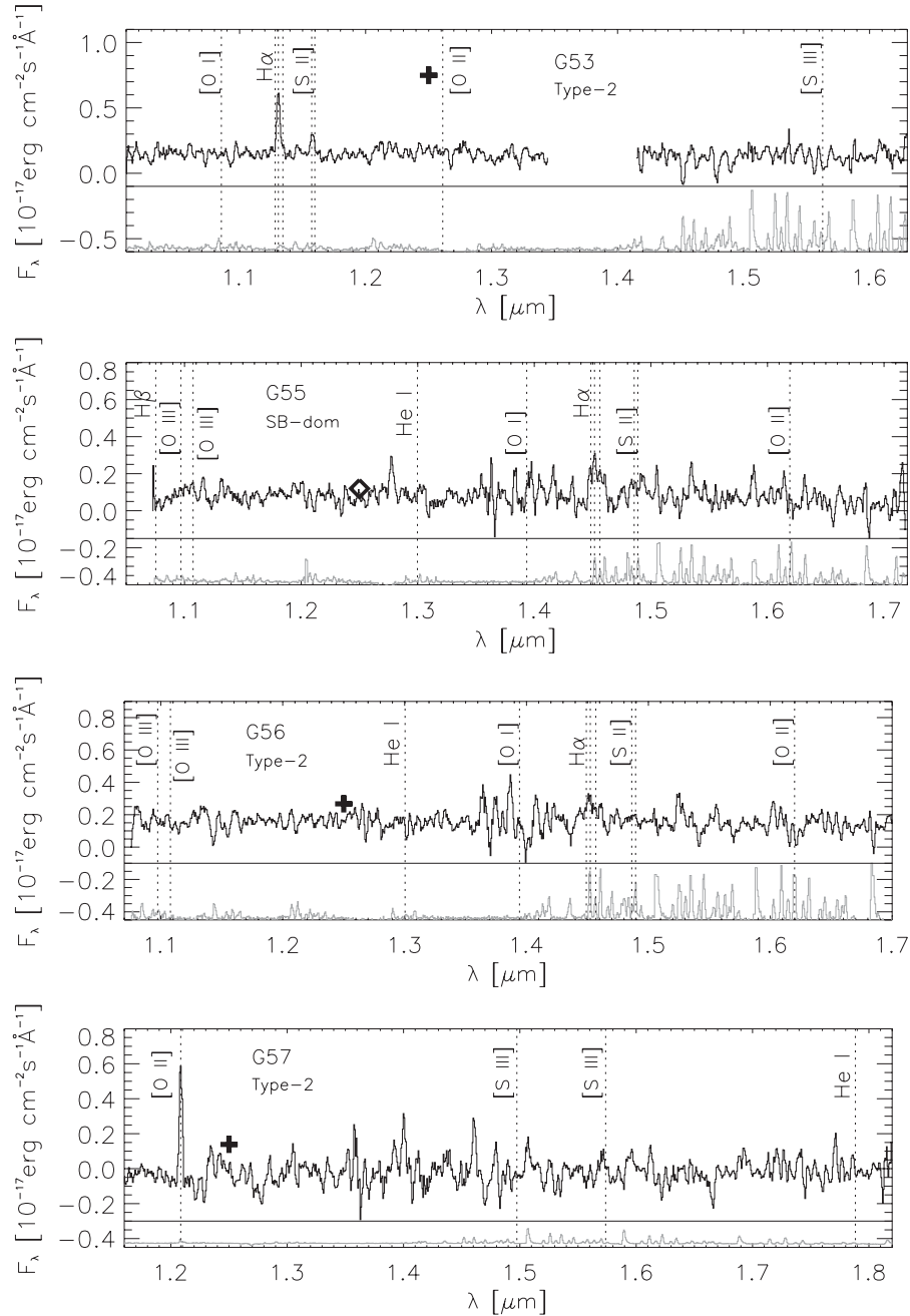
Figure 6. Same as in Fig. 4 but for the galaxies G53, G55, G56 and G57.
